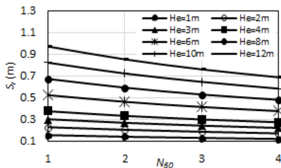
Figure 4: N_{60} Vs S_r for H_s/H_e=3 , LL=40 , e_0=0.8
