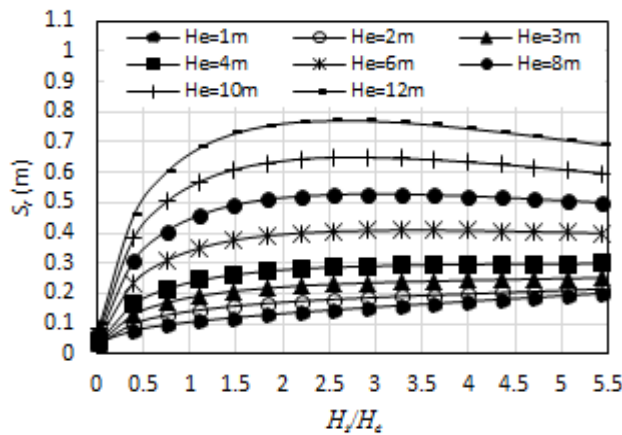
Figure 16: H_i/H_e Vs S_i for N_{d0}=3 , CR=0.19 , B_f=50m
