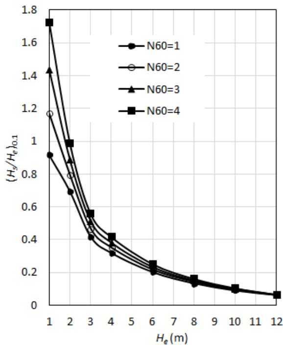
Figure 20: (H_s/H_e)_{0.1} Vs H_e to satisfy S_r \leq 0.100\text{m} for CR \leq 0.13 and B_i \leq 50\text{m}
