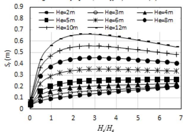
Figure 18: H_i/H_e Vs S_i for N_{d0}=4 , CR=0.16 , B_f=50m
