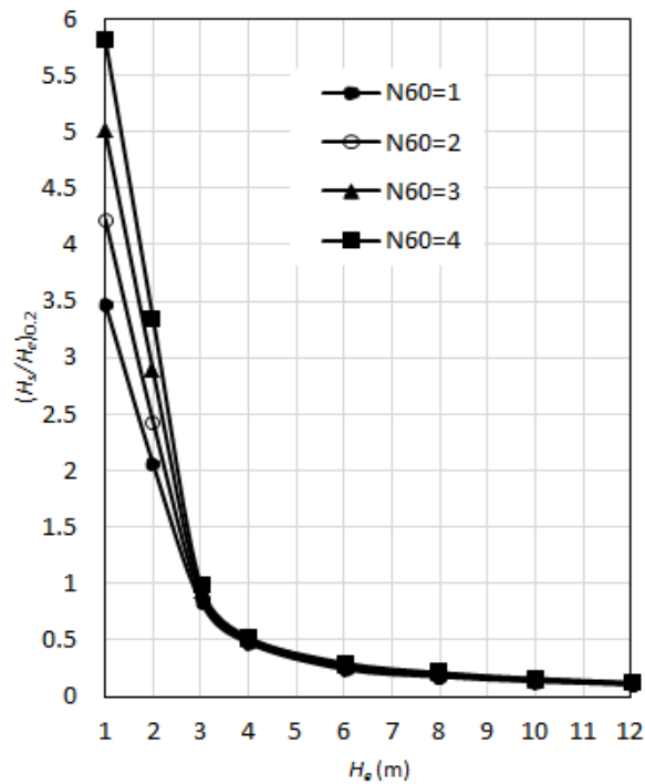
Figure 23: (H_s/H_e)_{0.2} Vs H_s to satisfy S_r=0.200m for 0.13 < C_d/(1+e_0) \leq 0.21 and B_s \leq 50m
