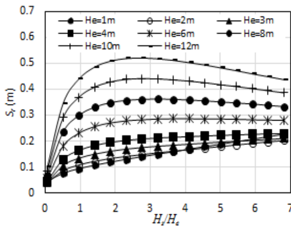
Figure 8: H/H_e Vs S_r for N_{60}=1 , CR=0.19 , B_f=50m
