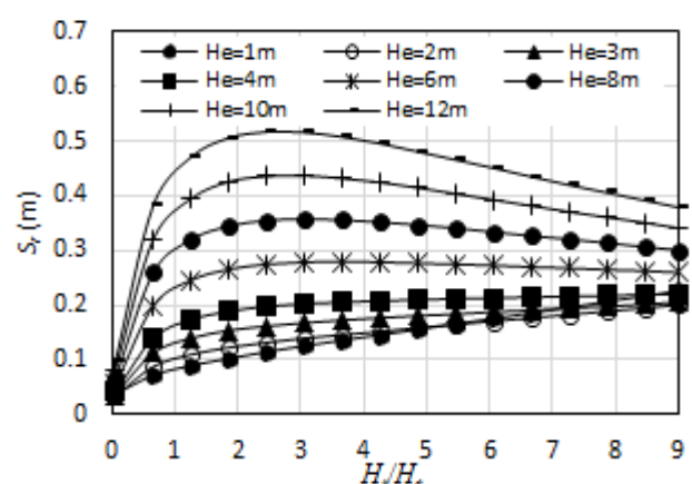
Figure 17: H_i/H_e Vs S_i for N_{d0}=4 , CR=0.21 , B_f=50m
