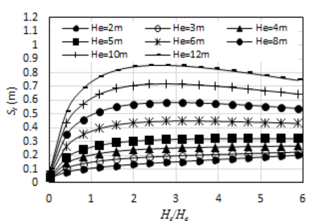
Figure 19: H_i/H_e Vs S_i for N_{d0}=4 , CR=0.21 , B_f=50m
