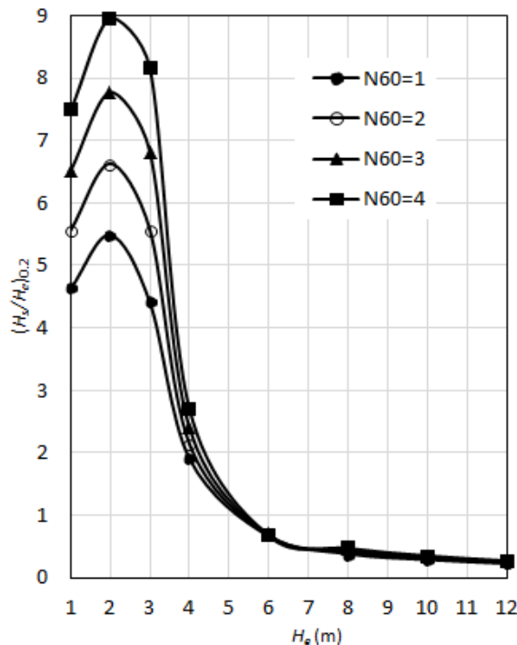
Figure 22: (H_s/H_e)_{0.2} Vs H_s to satisfy S_r=0.200m for C_d/(1+e_0) \leq 0.13 and B_s \leq 50m
