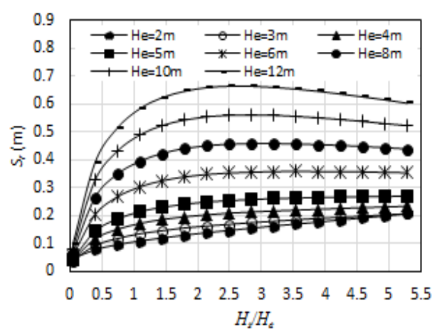
Figure 9: H/H_e Vs S_r for N_{60}=1 , CR=0.21 , B_f=50m
