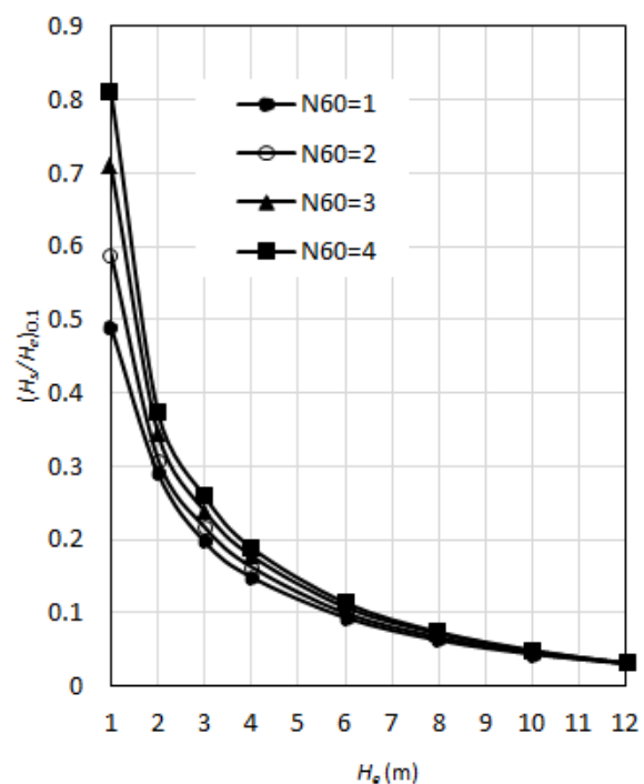
Figure 21: (H_s/H_e)_{0.1} Vs H_e to satisfy S_r \leq 0.100\text{m} for 0.13 < CR \leq 0.21 and B_i \leq 50\text{m}
