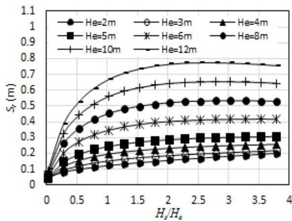
Figure 8: H/H_e Vs S_r for N_{60}=1 , CR=0.19 , B_f=50m
