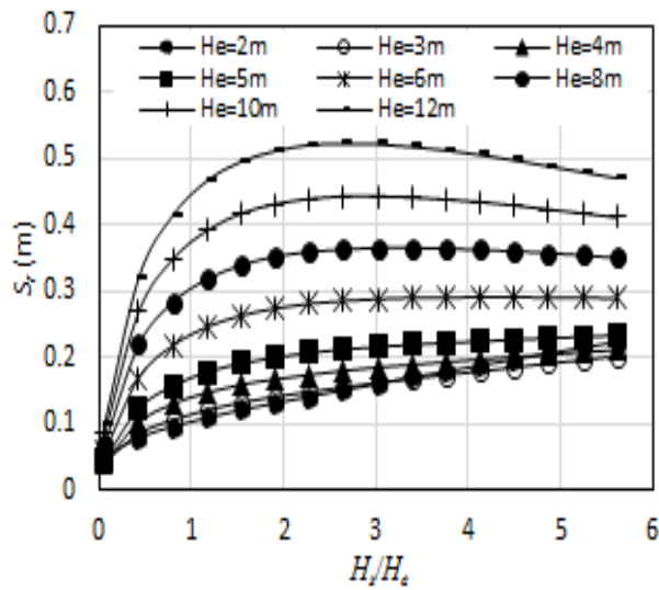
Figure 6: H/H_e Vs S_r for N_{60}=1 , CR=0.13 , B_f=50m
