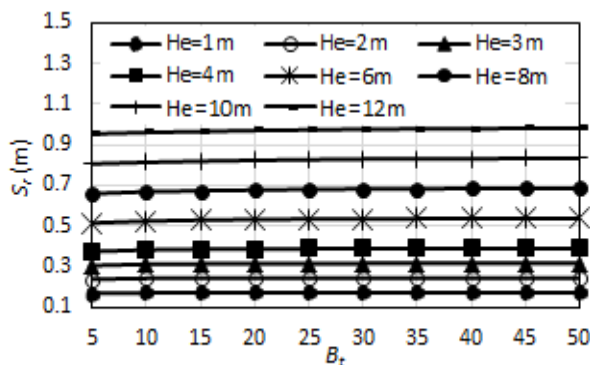
Figure 2: B_f Vs S_r for H_s/H_e=3 , N_{60}=1 , CR=0.11
