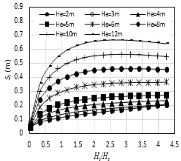
Figure 7: H/H_e Vs S_r for N_{60}=1 , CR=0.16 , B_f=50m
