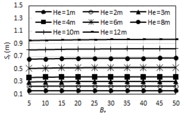
Figure 3: B_f Vs S_r for H_s/H_e=3 , N_{60}=1 , CR=0.16
