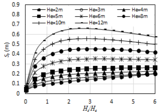
Figure 15: H_i/H_e Vs S_i for N_{d0}=3 , CR=0.16 , B_f=50m
