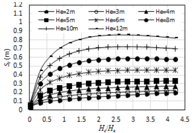
Figure 13: H_i/H_e Vs S_i for N_{d0}=2 , CR=0.21 , B_f=50m
