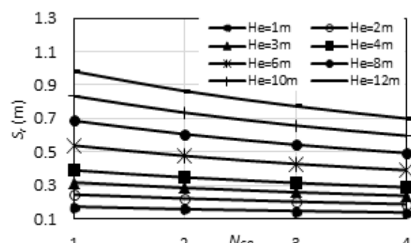
Figure 5: N_{60} Vs S_r for H_s/H_e=4 , LL=60 , e_0=1.2
