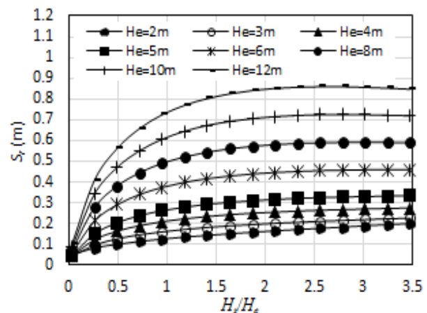
Figure 9: H/H_e Vs S_r for N_{60}=1 , CR=0.21 , B_f=50m
