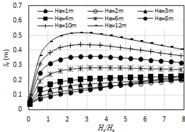
Figure 14: H_i/H_e Vs S_i for N_{d0}=3 , CR=0.13 , B_f=50m
