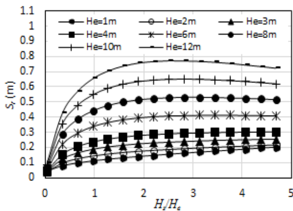
Figure 12: H_i/H_e Vs S_i for N_{d0}=2 , CR=0.19 , B_f=50m
